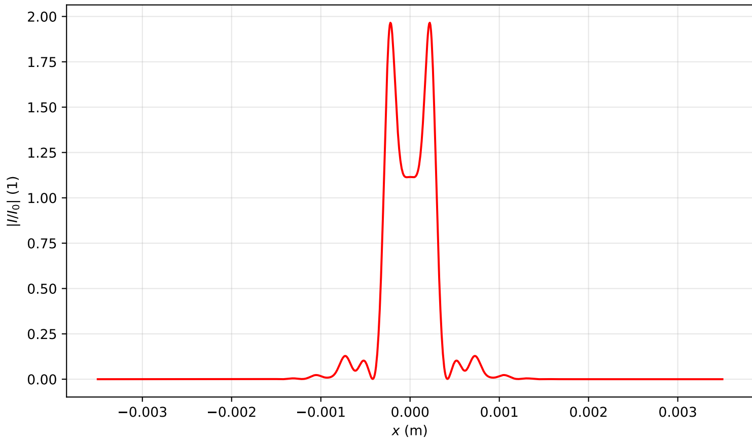
Intensity profile I(x, y = 0, z = 0.716)/I_0 , P_{in}=7.0P_{cr} , artificial time
